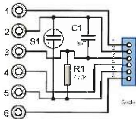
Figure 2: Access Provider Master Socket Circuit Diagram
